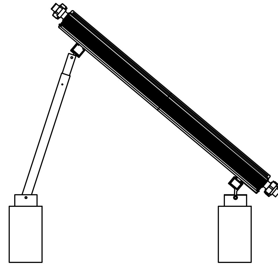
VIEW3 SCALE 1 / 10
